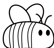
bee
