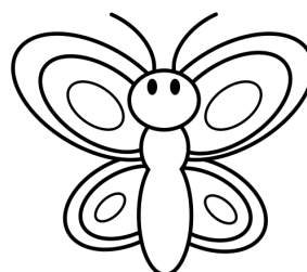
butterfly
