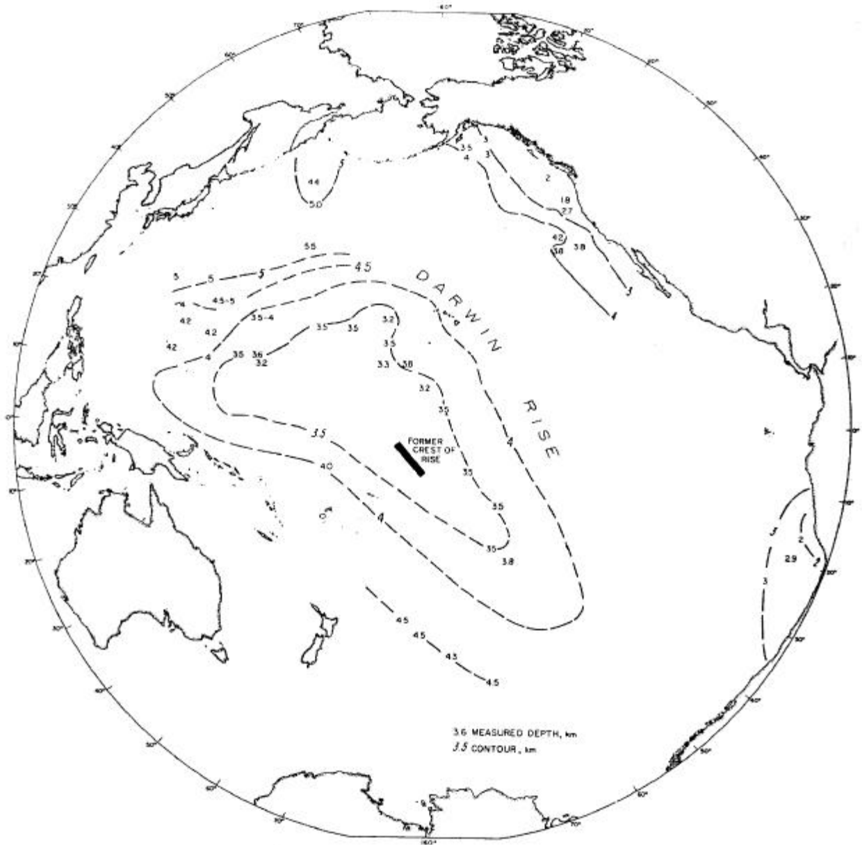
Figure 6.15 Paleobathymetry of Pacific Basin. (See text for mode of construction.) Contours shown are all shallower than at present, but not necessarily contemporaneous except on Darwin Rise.
